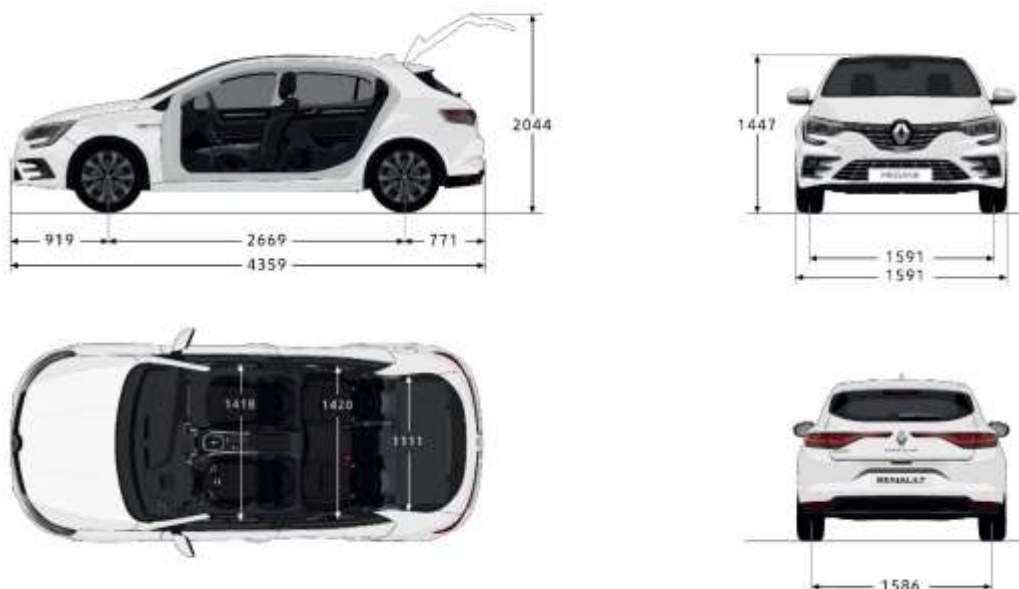
Dimensions (mm)
