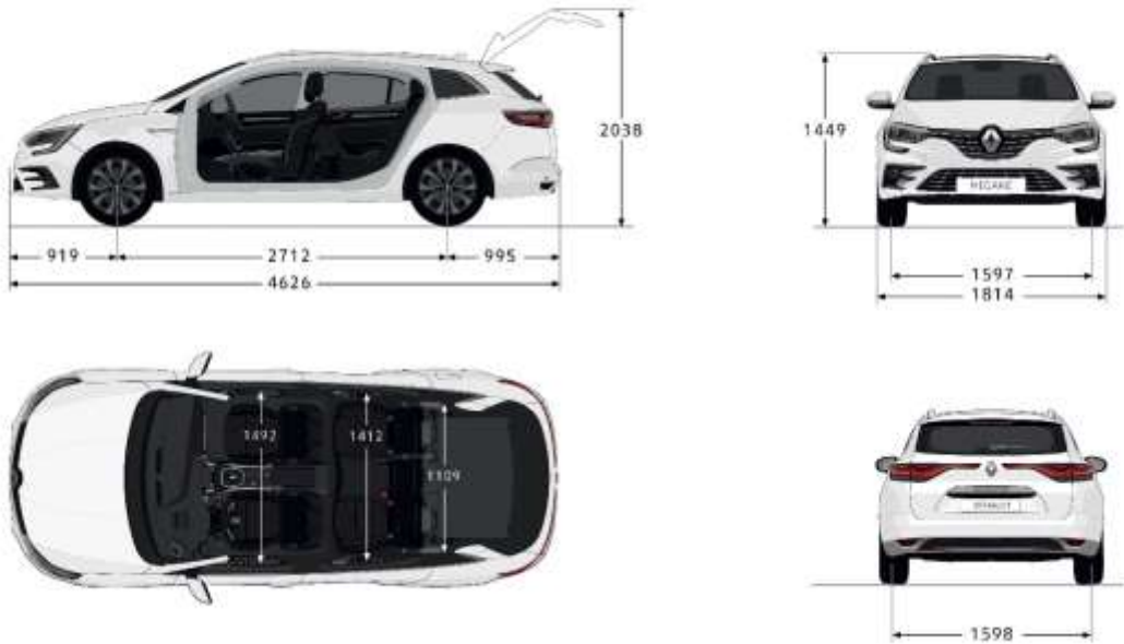
Dimensions (mm)
